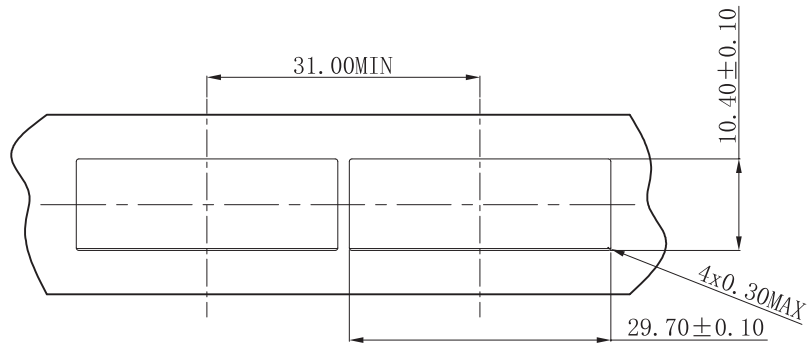
RECOMMENDED BEZEL CUT-OUT SINGLE SIDED APPLICATIONS
