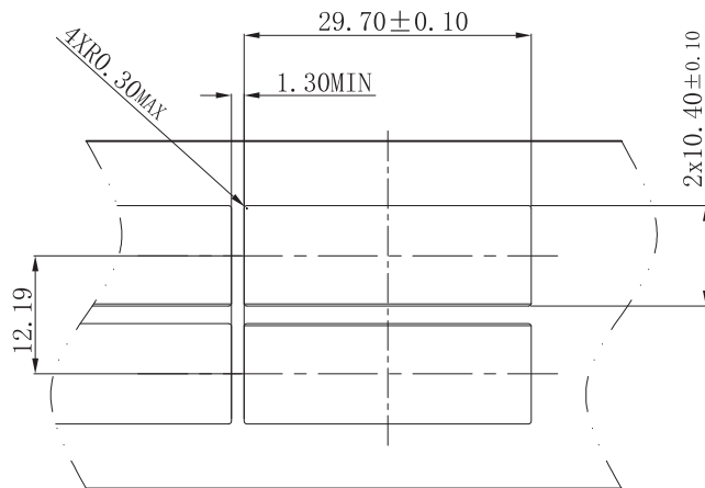
RECOMMENDED BEZEL CUT-OUT SINGLE SIDED APPLICATIONS
