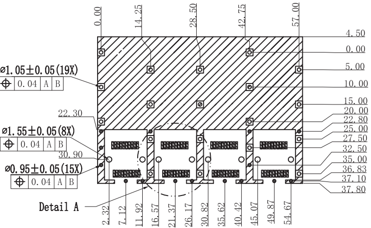
PCB LAYOUT THICKNESS=3.0MM (TOP VIEW)
