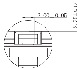
DETAIL C SCALE 4:1
