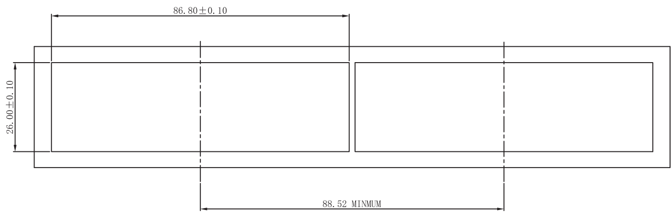
BEZEL CUT-OUT CENTER SPACING DETAIL BEZEL THICKNESS:0.8-2.6
