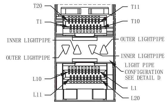
DETAIL A1 SCALE 2:1
