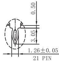
DETAIL B SCALE 5:1
