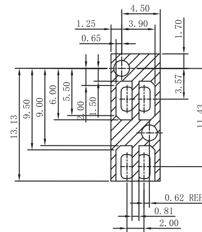
KEEPOUT ZONE DETAIL SCALE 5:1
