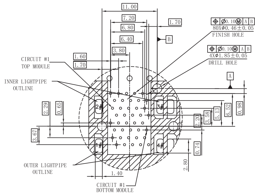
DETAIL F SCALE 5:1
