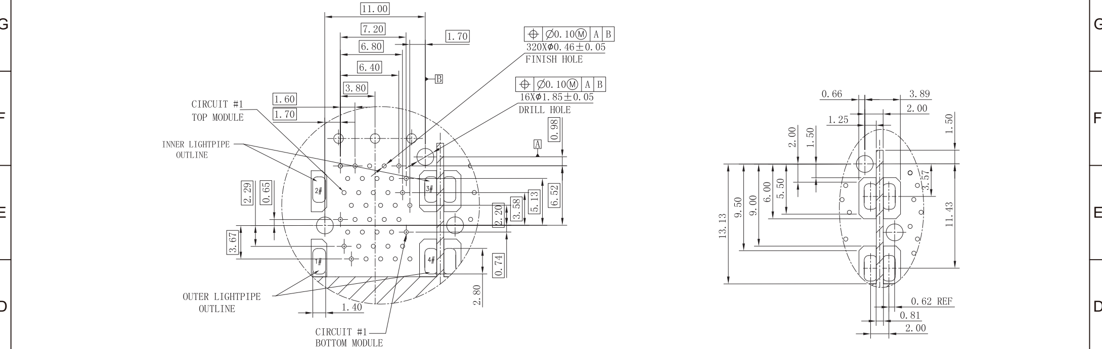
KEEPOUT ZONE DETAIL SCALE 5:1
